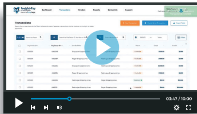
Freight-Pay overview
